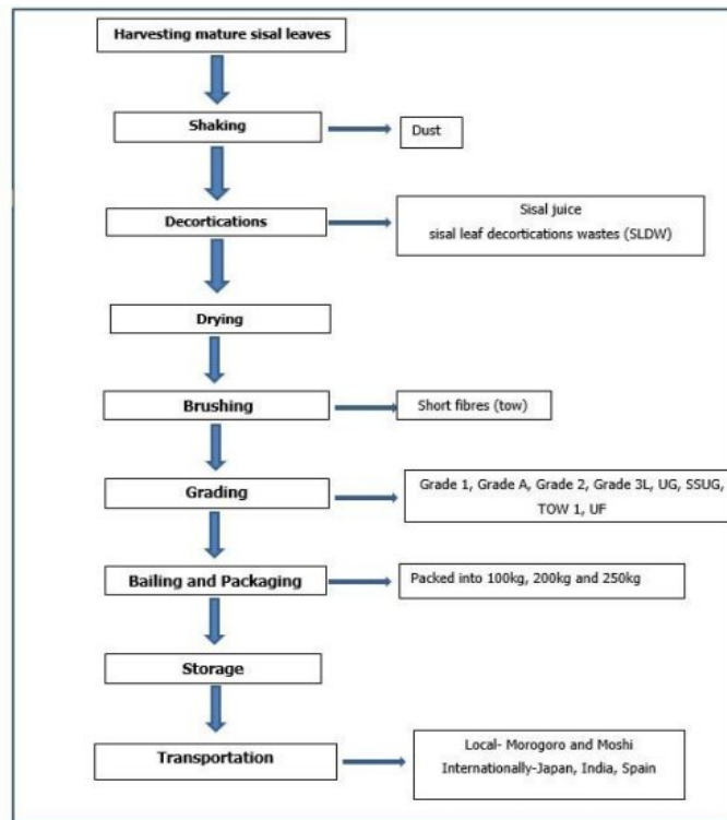
Figure 2: Production Process flow chart
