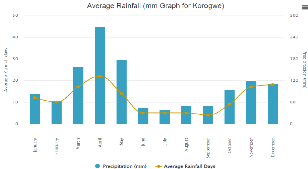
Figure 6; Rainfall averages
