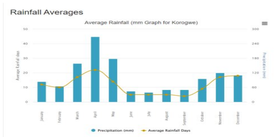
Figure 5; Rainfall averages
